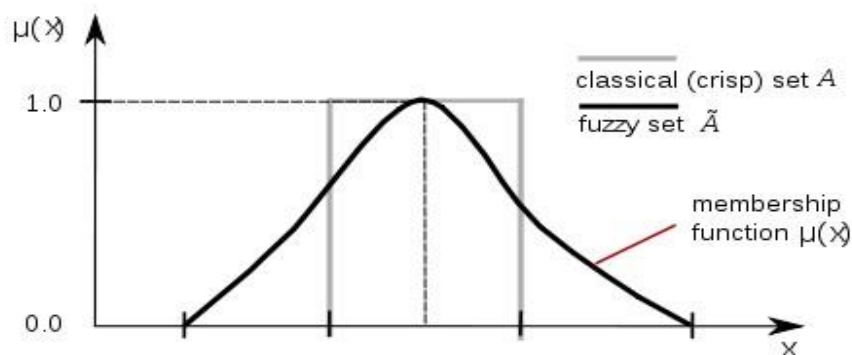
Figure. 1: Membership function of a fuzzy set (Aliev et al. , 2015b)
