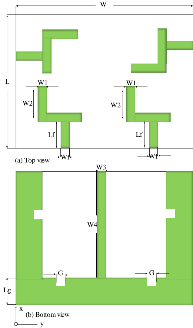
Figure 1. 4 x 4 MIMO Antenna Geometry
