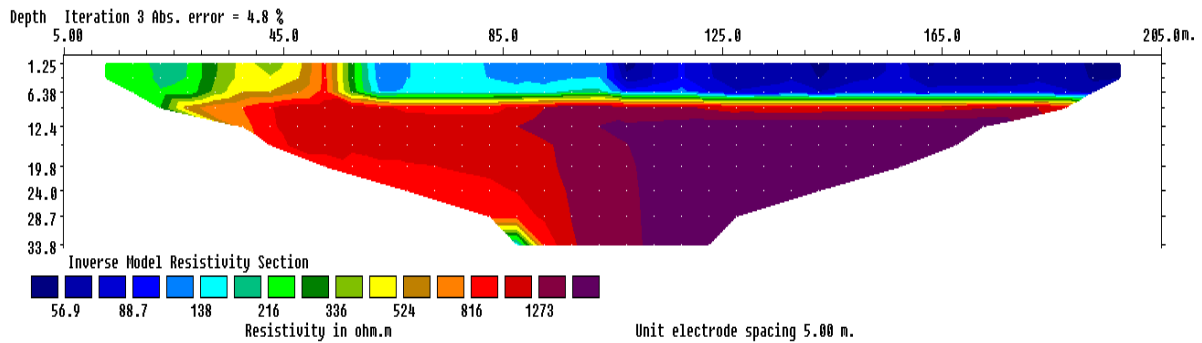
Figure 10: Results of 2D Inversion of Wenner array along Profile 5
