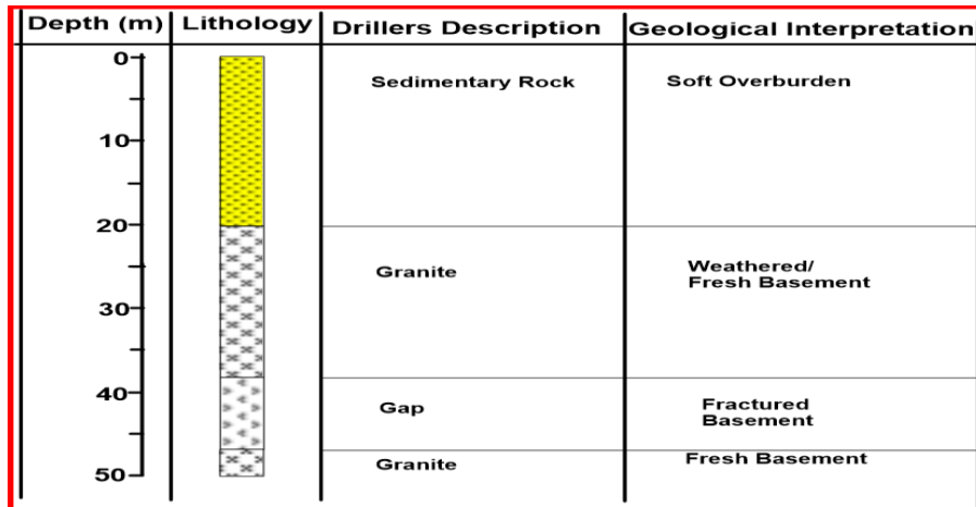
Figure 5: Geological Correlation of Drillers Log with Data from this Study (Modified from China Zhongao Nigeria LTD, 2010)
