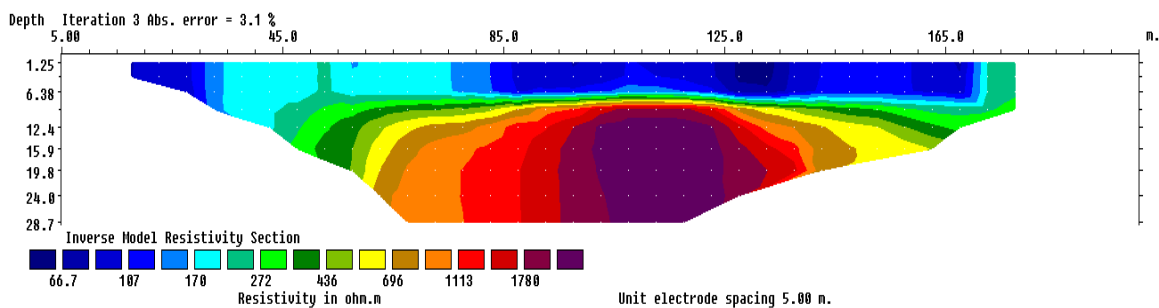
Figure 8: Result of 2D Inversion of Wenner Array along Profile
