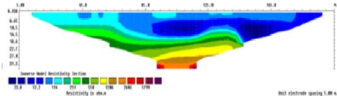
Figure 6: Results of 2D inversion of Wenner Array along Profile 1
