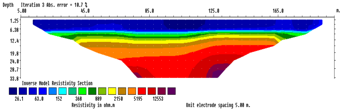
Figure 6: Results of 2D inversion of Wenner Array along Profile 1
