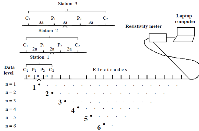
Figure 3: The Arrangement of Electrodes for a 2D Electrical survey and the sequence of Measurements used to build up a pseudo section.
