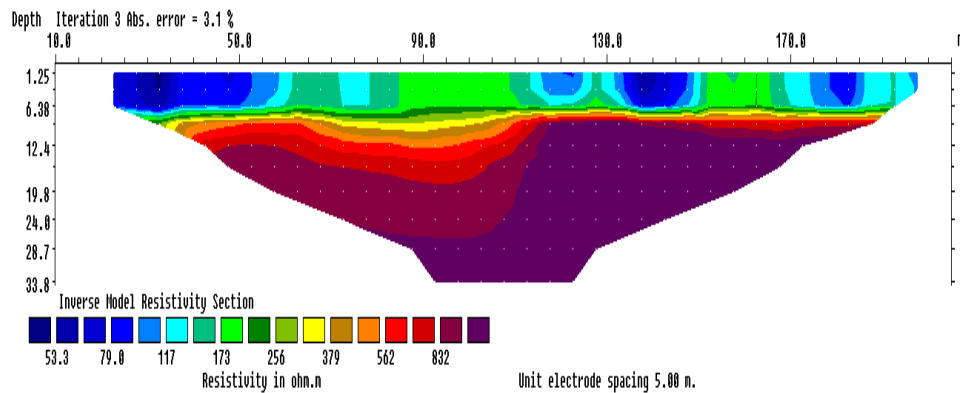
Figure 8: Result of 2D Inversion of Wenner Array along Profile
