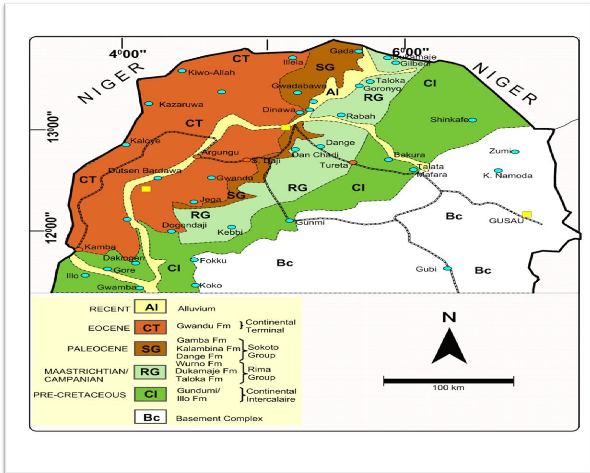
Figure 1: Generalized Geological Map of Sokoto, (Modified After Obaje et al. , (2013)
