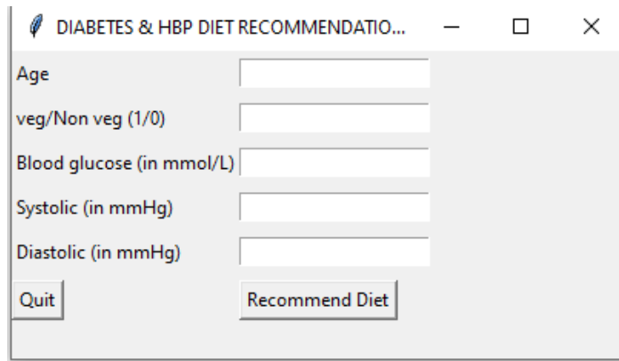
Figure 7: User interface of the recommender system
