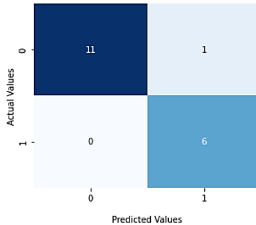
Figure 10: Confusion matrix
