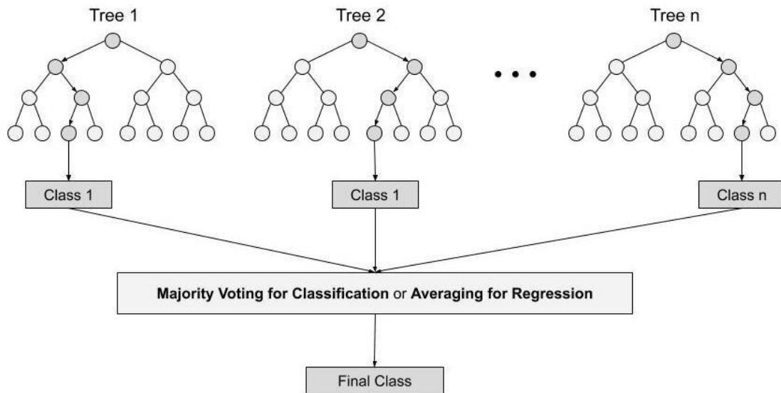
Figure 4: Random Forest (source: Analytic Vidhya, 2022)
